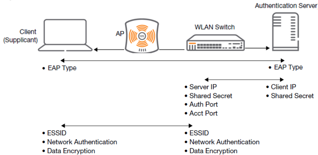
Figure 32 802.1X Authentication with a RADIUS Server
