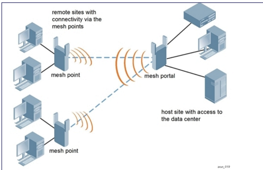
Figure 83 Sample Point-to-Multipoint Deployment
