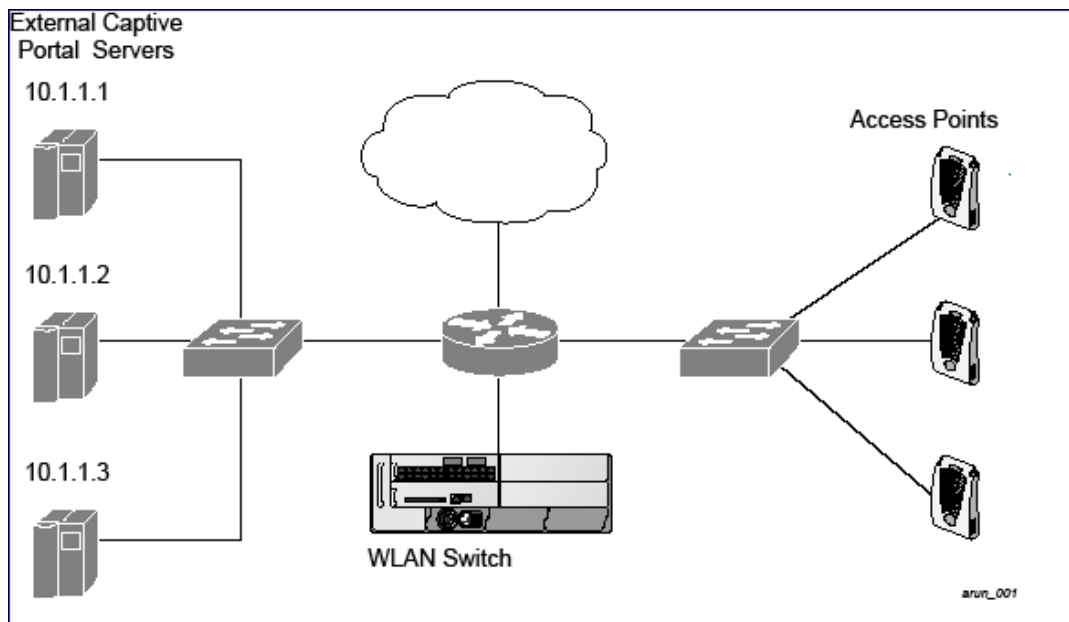
Figure 118 Example NAT-Mode Topology
