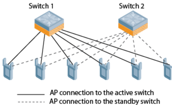
Figure 86 1:1 Active/Standby Deployment
