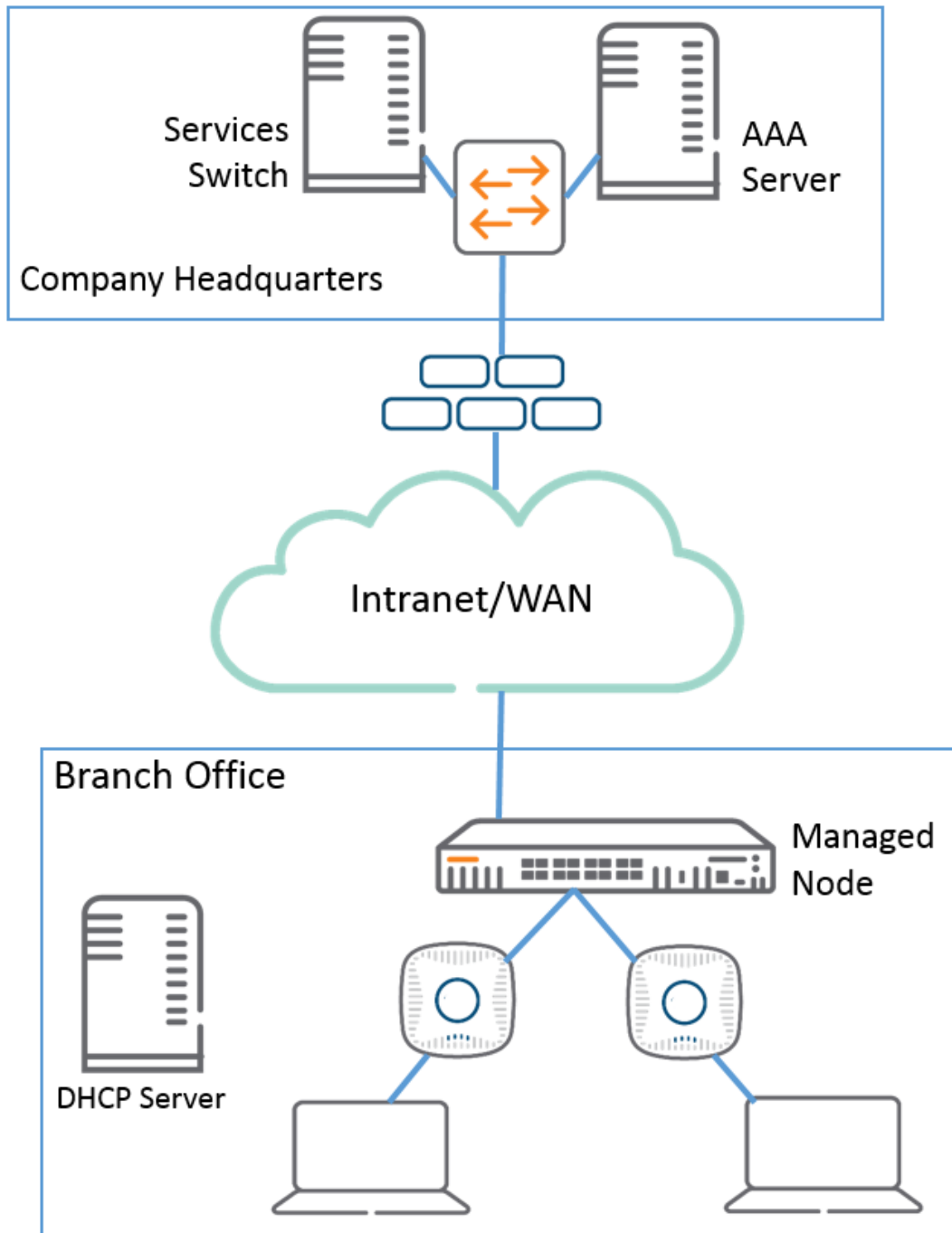
Figure 28 Managed Device Topology
