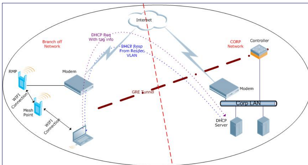
Figure 80 Working of Remote Mesh Portal
